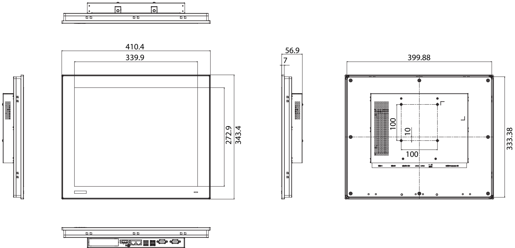
Panel Cutout Dimensions: 401.3 x 334.8 mm (15.80" x 13.18")
