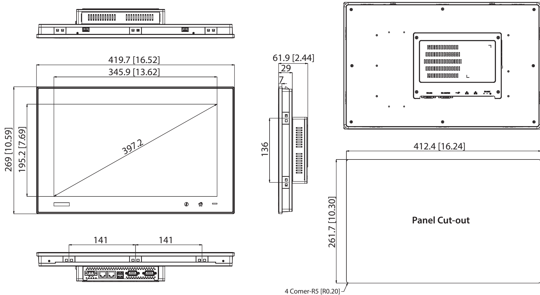
TPC-1551WP Panel Cut-out Dimensions: 412.4 x 261.7 mm
