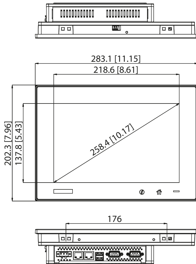
TPC-1051WP Panel Cut-out Dimensions: 274.6 x 193.8 mm
