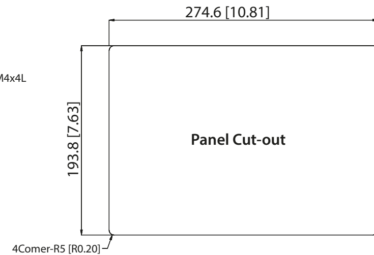
TPC-1051WP Panel Cut-out Dimensions: 274.6 x 193.8 mm
