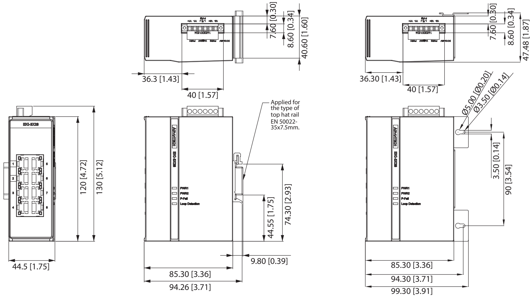
DIN-rail Mounting
